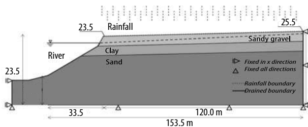
Figure 2. Cross section of the layered embankment and its boundary conditions
