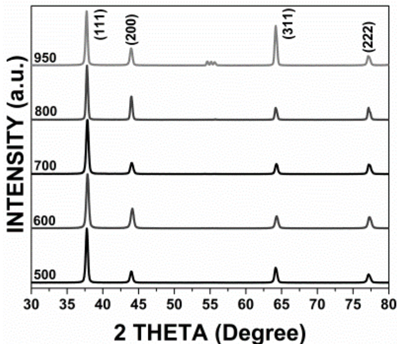
Figure 2. Superposition of X-ray Diffraction Pattern.
